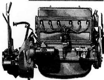
1928 CHEVROLET 5-CYLINDER VALVE-IN-HEAD ENGINE
